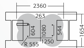
Supported area of the swivel arms in mm
