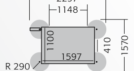
Supported area of the swivel arms in mm HM 1100-04
