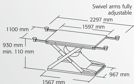
Supported area of the swivel arms in mm HM 1100-04
