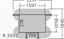
Supported area of the swivel arms in mm HM 1100-04
